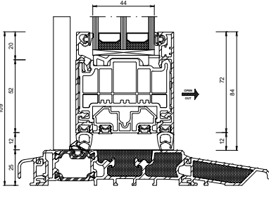
Low Threshold
