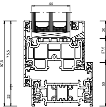
Outer Frame
