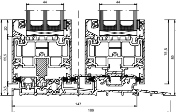
Treshold
